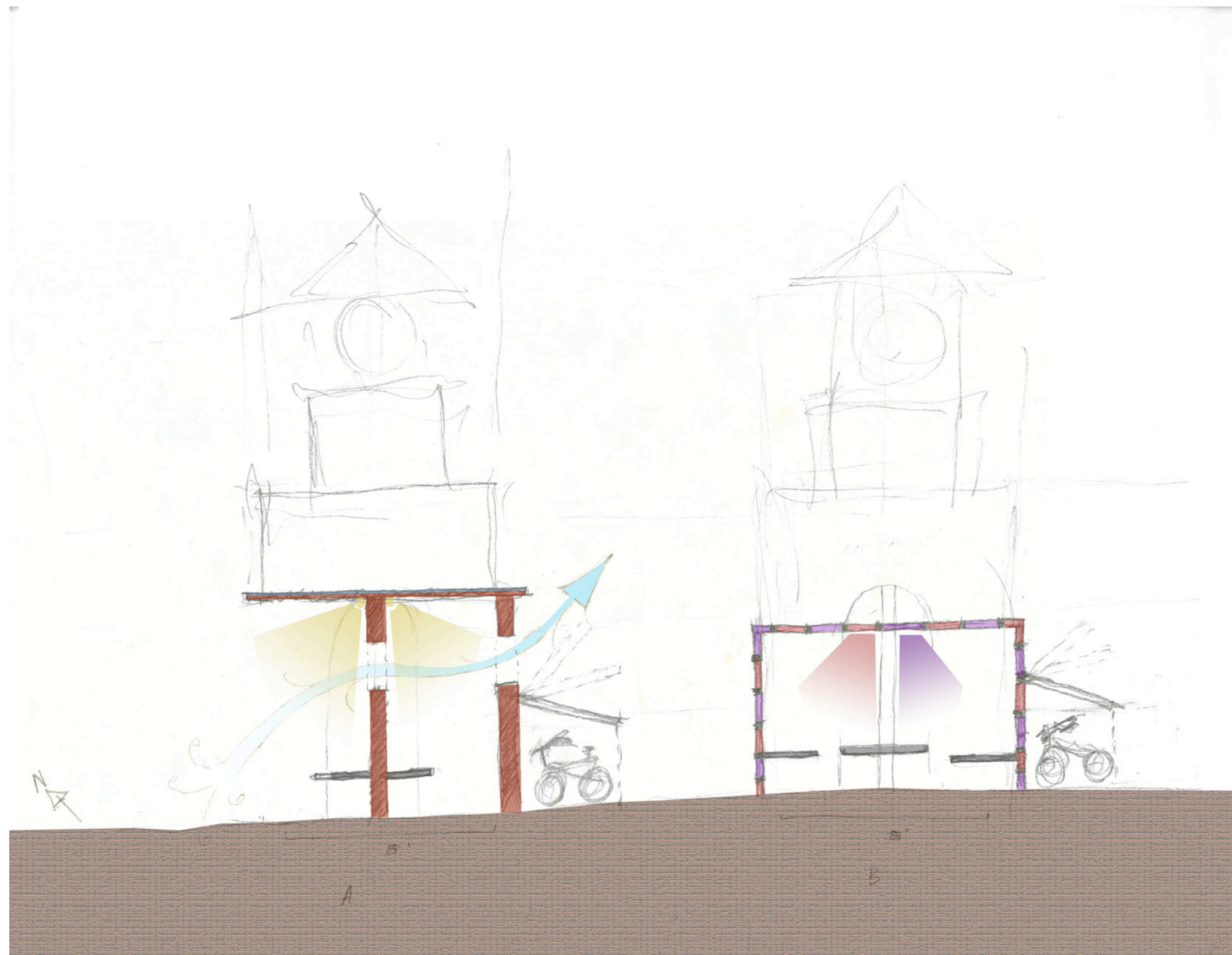
Transverse Section and Wind Diagram
